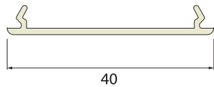
40mm Light Diffuser
