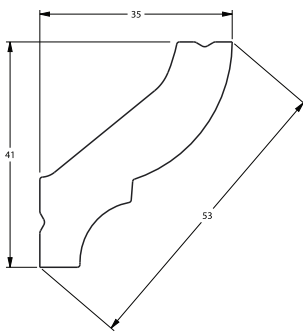
CORNICE MOULDING CB502N
