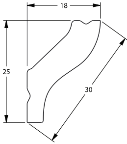
CORNICE MOULDING CB501N
