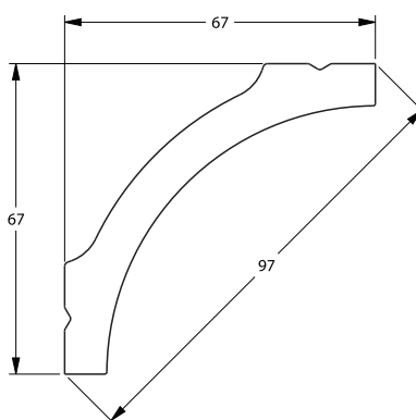
CORNICE MOULDING CB522N
