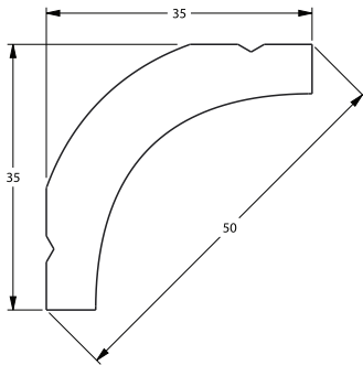
CORNICE MOULDING CB520N
