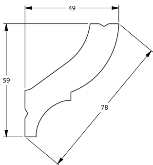
CORNICE MOULDING CB503N
