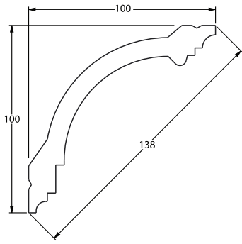
CORNICE MOULDING CB512N
