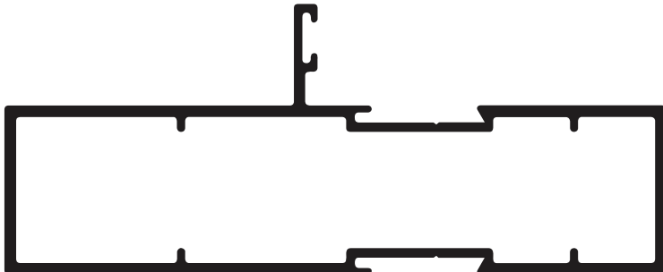
Glazing 4 (Double Lip)
